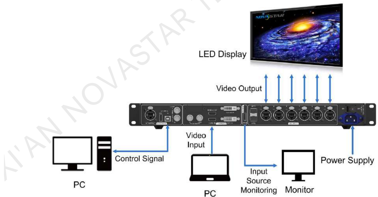
Figure 3-1 Application of sending card mode
