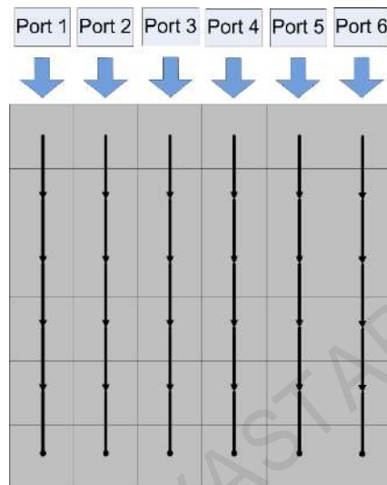
Figure 7-9 Each Ethernet port loading only one column of cabinets
