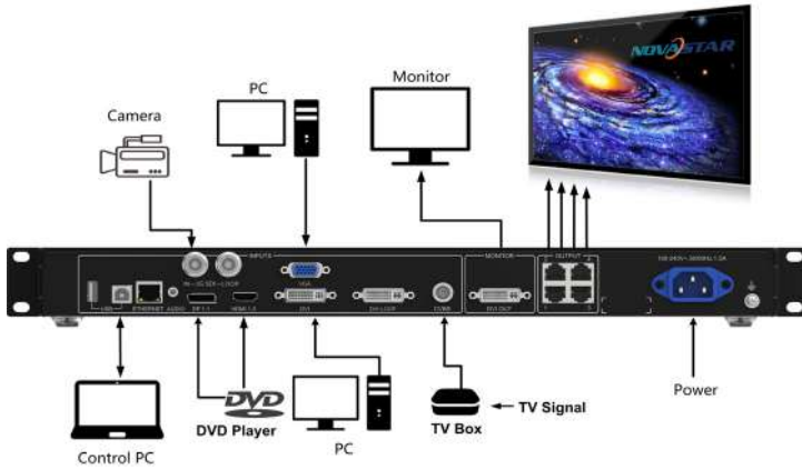
Signal connections
